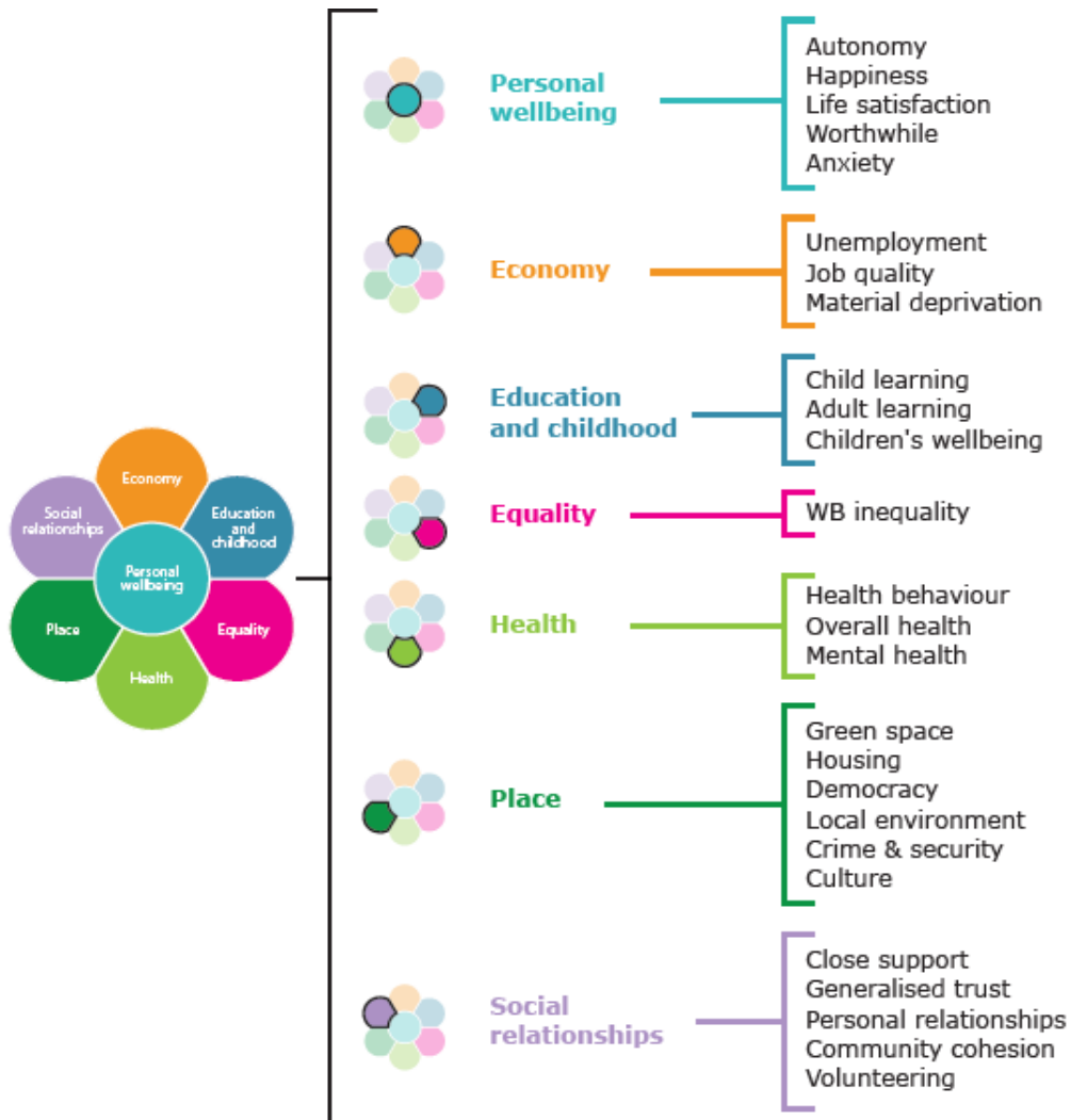
Figure 3: Sub-domains
