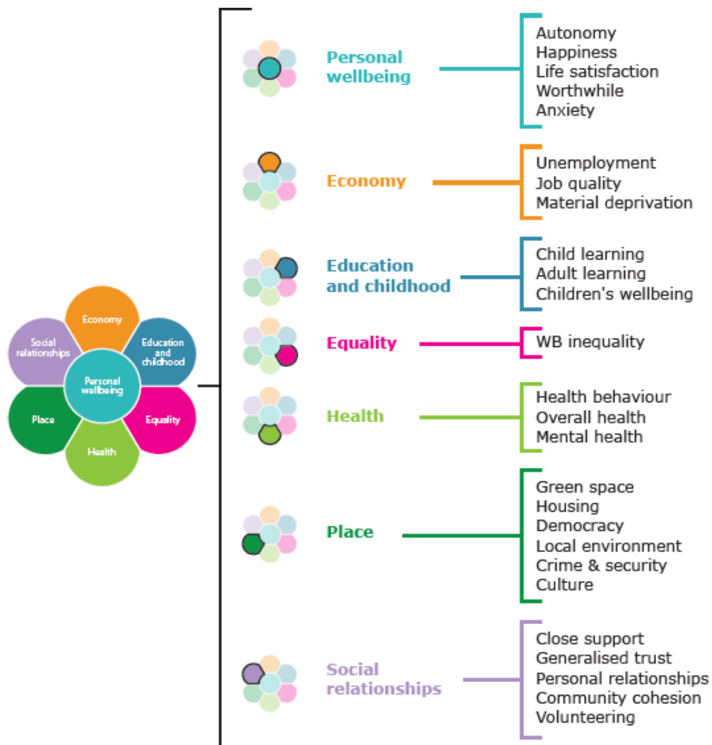
Figure 3: Sub-domains
